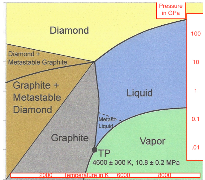
Figure 9d: Theoretical carbon phase diagram from [Wikimedia (2017)]. Note that this reference claims that considerable disagreement exists between theory and experiment.
