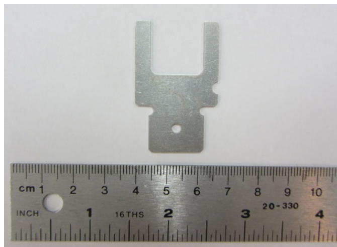
Fig. 10c. Top view of Type ACF-F30 mod. 2 fork. Customer specifies whether foil is mounted on top or bottom.
