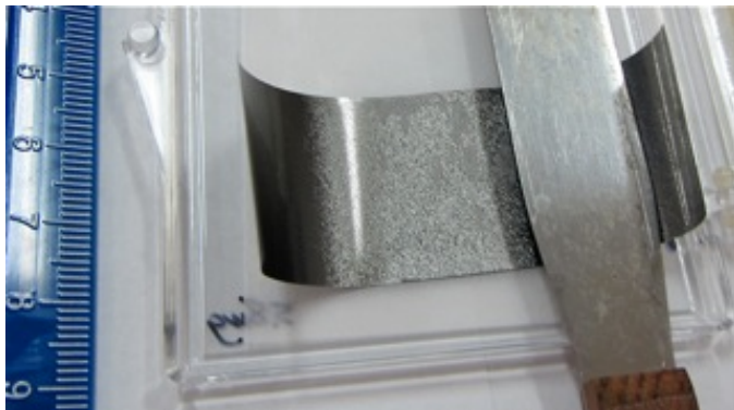
Fig. 2. Evaporated carbon foil (approx. 80 \mu\text{g}/\text{sq.cm} , 25 mm x 68 mm) removed from its substrate. The tendency to curl indicates residual stresses in the foil (see section 2.5 below):
